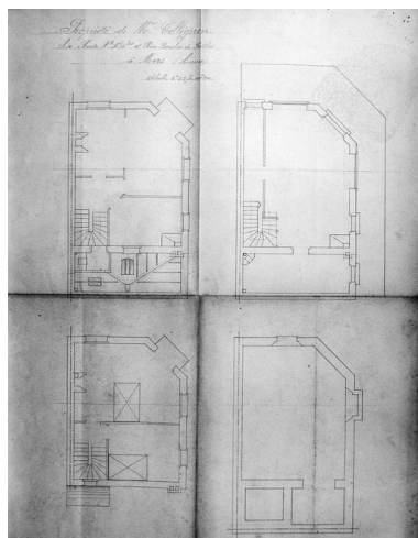
Plans des niveaux, [s.n.], [s.d.] (AC Mers-les-Bains). Phot. Leullier Irwin IVR22_20008000601XB
